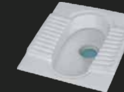
ORP - 04 - MD PAN Squatting Pan 520 x 420 x 170 mm
